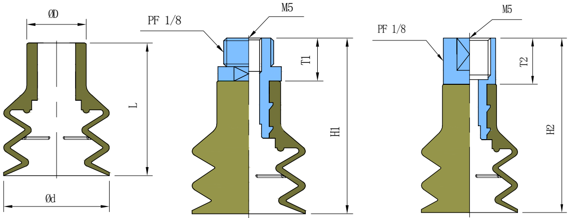
▶ 吸盘外形图/Dimensions
